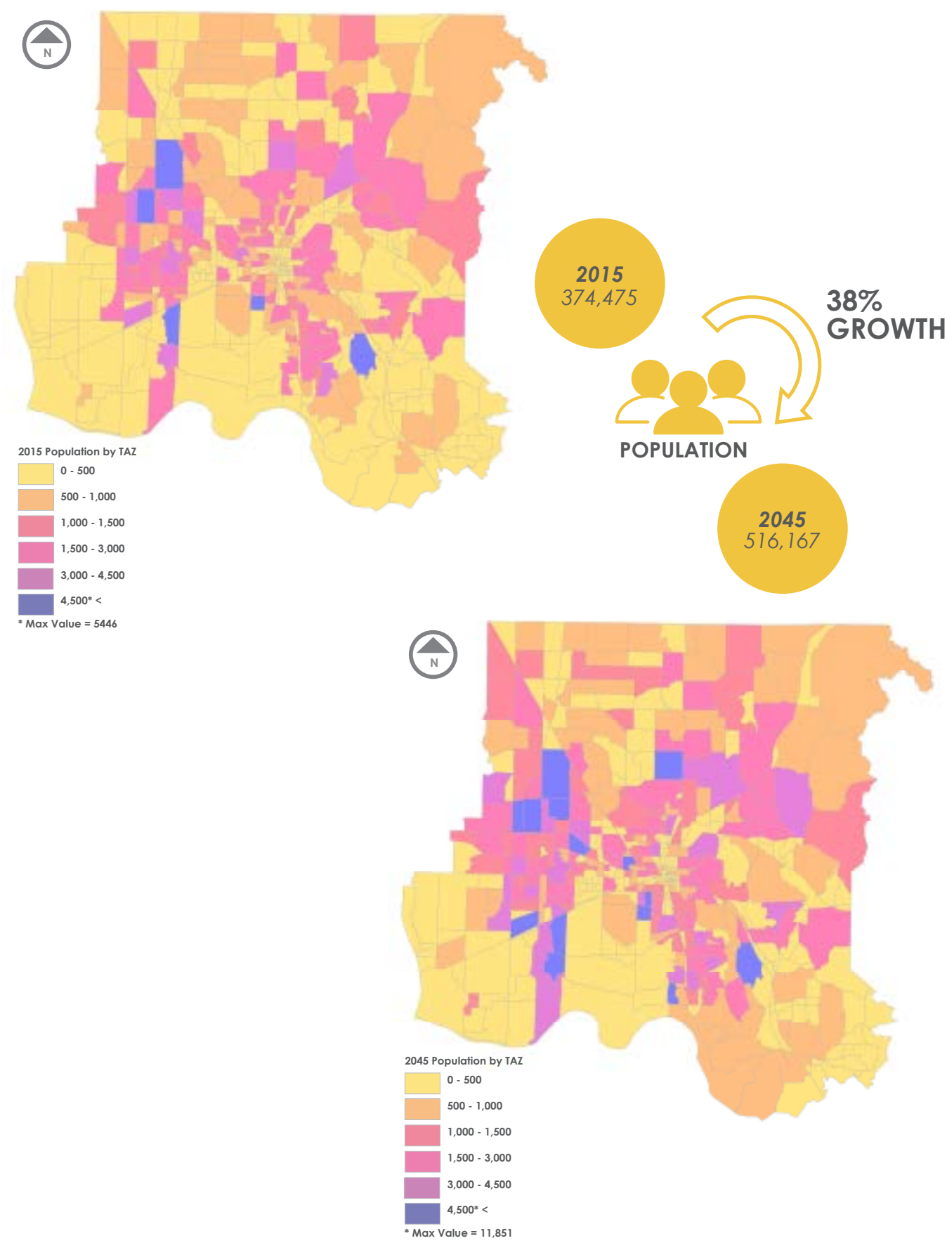
Map 3.1: Population Change 2015 - 2045
